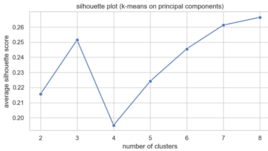
Figure 8: Silhouette plot for K-means on the first 5 principal components retained from the PCA.
